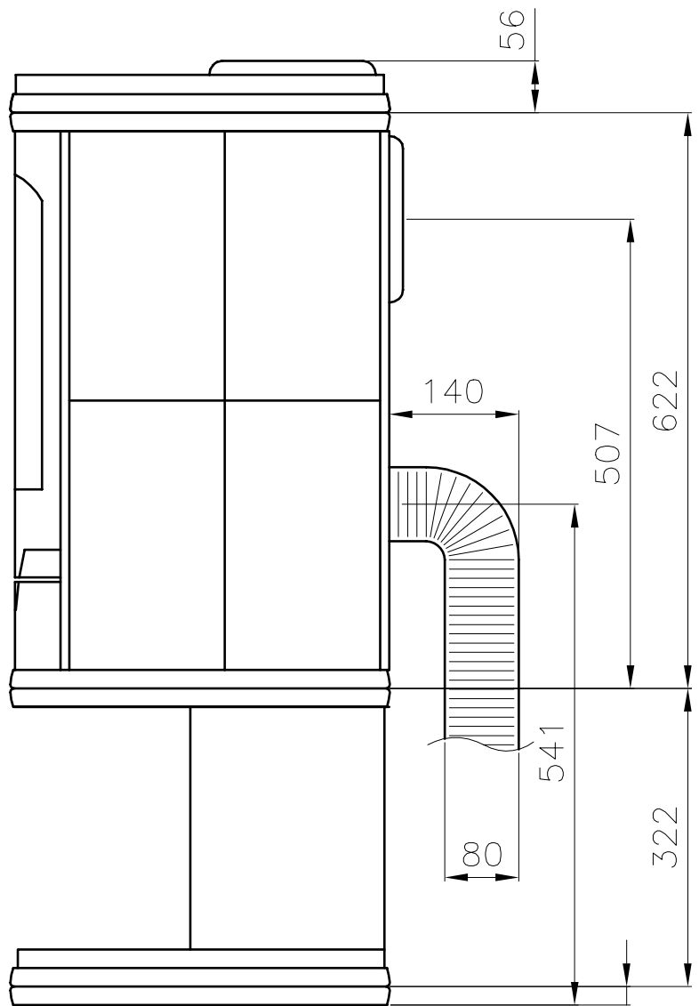
ECLIPS CONSOL
